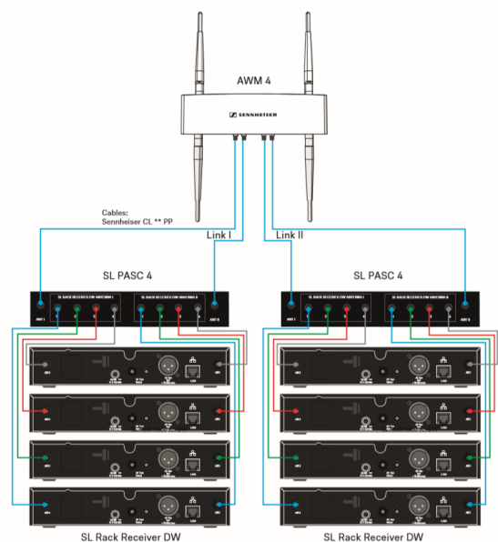
B: 8x SL Rack Receiver DW + AWM 4
