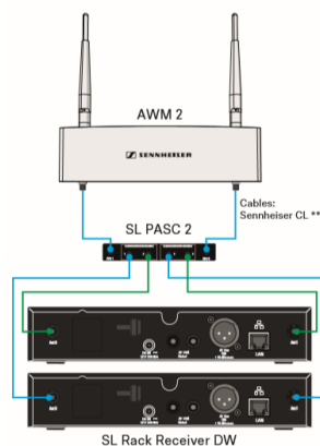
Example wiring diagrams for AWM2, AWM 4, PASC 2 and PASC4
