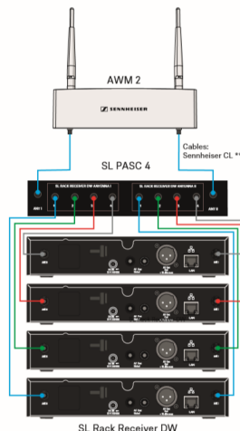
Example wiring diagrams for AWM2, AWM 4, PASC 2 and PASC4
